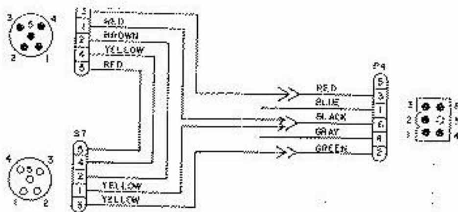
Schematic, Console Adapter 042776 (Plugs and Sockets Shown from Wire End)
