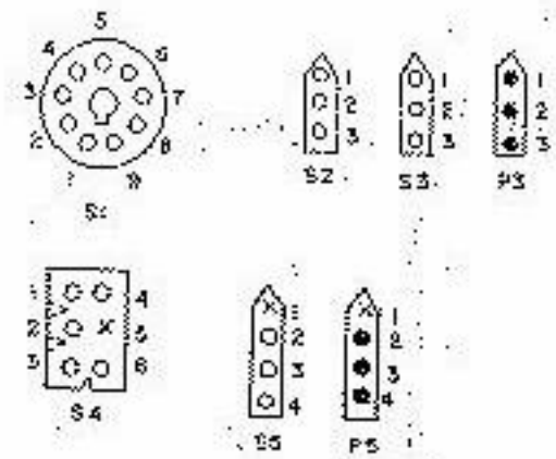
Plugs and Sockets (Shown from Wire End)
