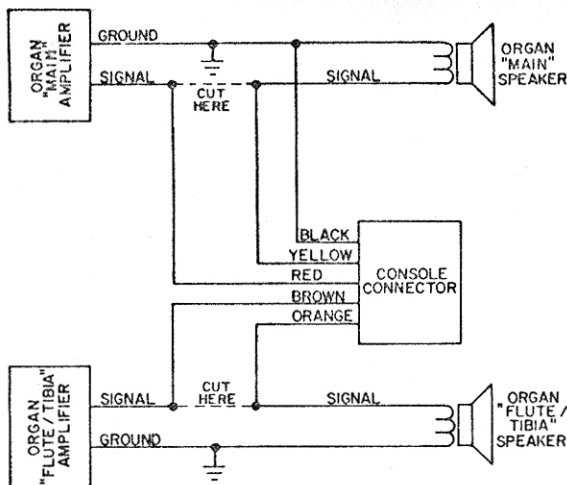
Figure 3. Interconnections, Two-speaker Organ
